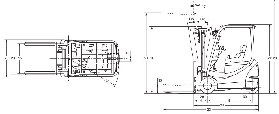
Dimensions/AM50 Series
