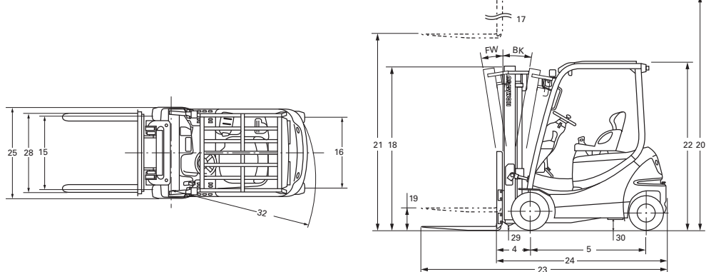
Dimensions/AE50 Series
